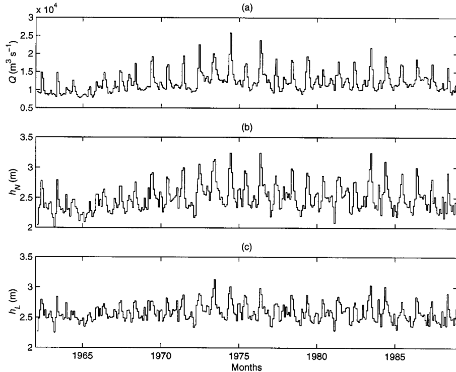
Fig. 2 DEF's monthly mean discharge at (a) the Québec-Lévis cross-section, and monthly mean water level, at (b) Neuville, and (c) Lauzon, from January 1962 to December 1988.
