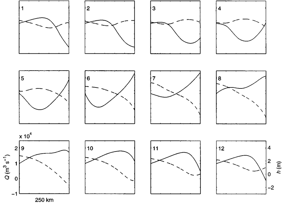
Fig. B2 Discharge (solid line), and water level (dashed line) over a hypothetical canal of simple geometry, for each hour of a semi-diurnal tidal cycle. The model is forced at its upstream boundary with a constant discharge of Q(t) = 10^4 \text{ m}^3 \text{ s}^{-1} , and at its downstream boundary with a semi-diurnal cyclical variation of the water level.
