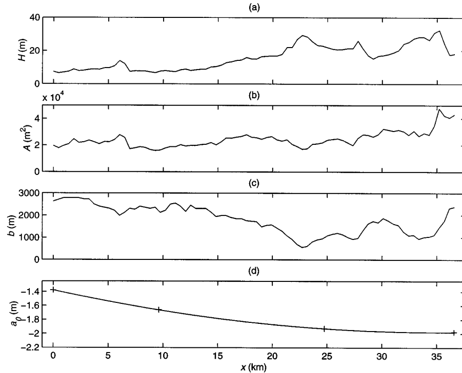
Fig. 4 Hydraulic characteristics for each of the 80 cross-sections that discretized the river between Neuville and Lauzon: (a) mean depth H ; (b) area A ; (c) surface width b ; (d) mean water-level relative to the International Great Lakes Datum 1985 a_0 . The mean water-level a_0 is interpolated at each grid cell from available measurements at Neuville, St. Augustin, Irving Wharf and Lauzon, identified by a plus sign on the figure.
