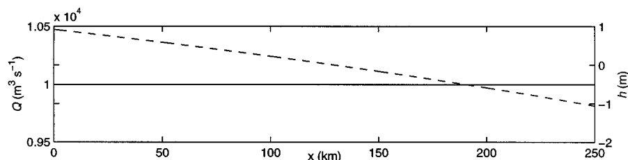
Fig. B1 Discharge (solid line) and water level (dashed line) over a hypothetical canal of simple geometry after steady state has been reached from a state at rest, and under steady boundaries forcing conditions ( Q(t) = 10^4 \text{ m}^3 \text{ s}^{-1} at both boundaries).
