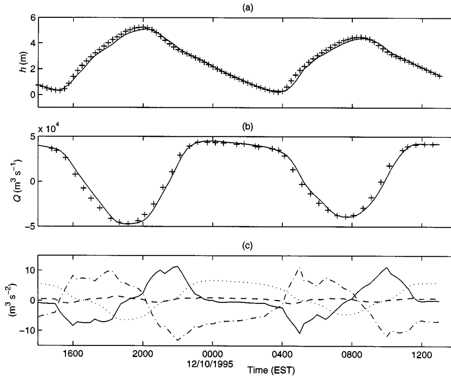
Fig. 5 (a) Comparison between observed (plus sign) and computed water level (solid line) at tidal gauge 3246 (Québec harbour). (b) Comparison between observed (plus sign) and computed discharge (solid line) at cross-section A (see Fig. 1). (c) Balance of terms of the momentum equation at cross-section A (solid line for the inertial term, dashed line for the advection term, dashed-dotted line for the pressure gradient, and dotted line for the bottom friction term).
