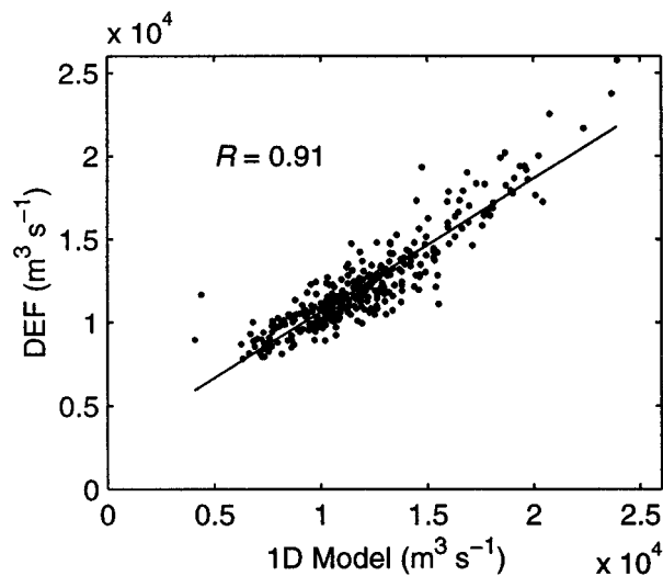
Fig. 7 DEF's mean monthly estimates versus monthly-averaged discharge from the 1D model. The solid line represents the least squares linear regression fit, along with the coefficient of correlation R = 0.91 . The few major outliers are attributed to errors in the interpolated data over missing segments.
