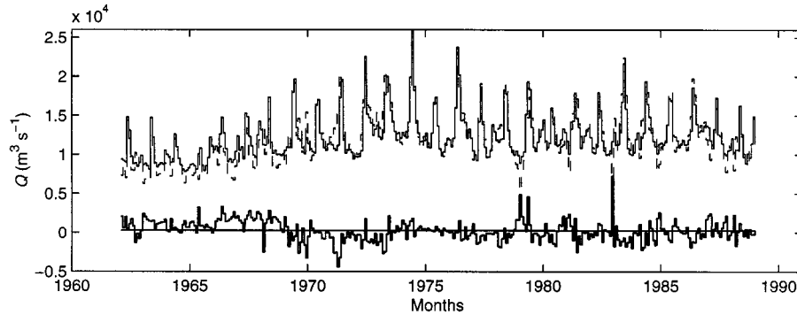
Fig. 6 Comparison between the DEF's monthly mean estimates (thin solid line), and monthly-averaged discharge from the 1D model (dashed line), along with the differences between the two methods (DEF minus 1D Model) (thick solid line), from January 1962 to December 1988.
