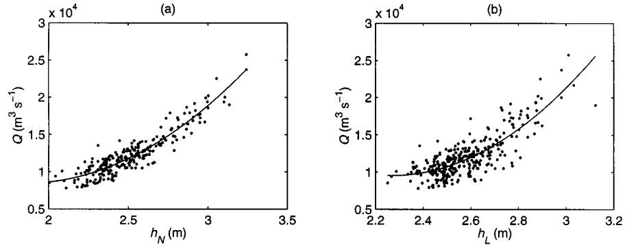
Fig. 3 DEF's monthly mean discharge plotted versus monthly mean water-level, at (a) Neuville and (b) Lauzon. The solid lines are the second-order polynomial least-squares fit as described by equations 1 and 2 respectively. Months with more than 10% missing data in the original water level series are discarded from the analysis, which results in 245 and 296 monthly averages for Neuville and Lauzon, respectively.
