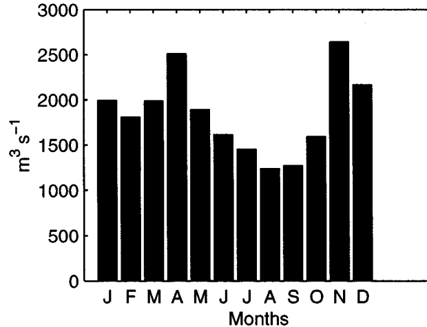
Fig. 8 Seasonal root-mean-square differences ( \text{m}^3 \text{s}^{-1} ) between DEF's estimates and monthly-averages from the 1D model. Statistics are computed from January 1962 to December 1988.
